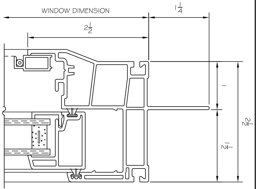
2 TYP. HEAD AT FIXED LITE
