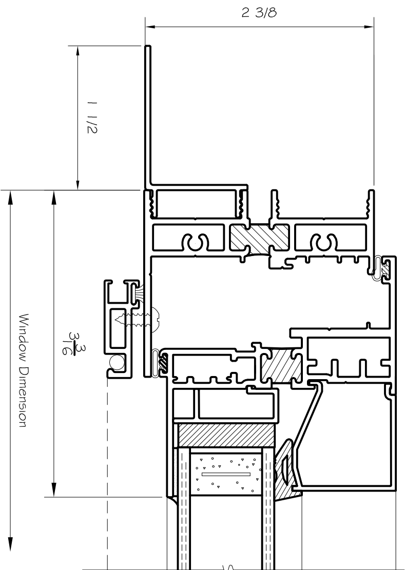
5 JAMB AT SASH W/ OPTIONAL NAILING FLANGE
