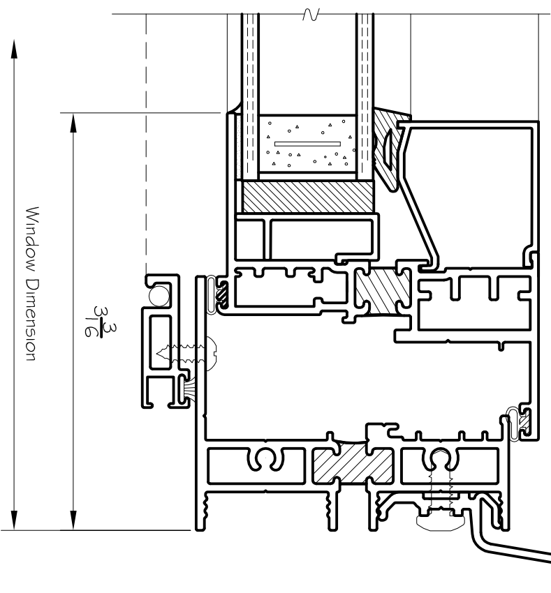
6 JAMB AT SASH W/ OPTIONAL STRAP ANCHOR
