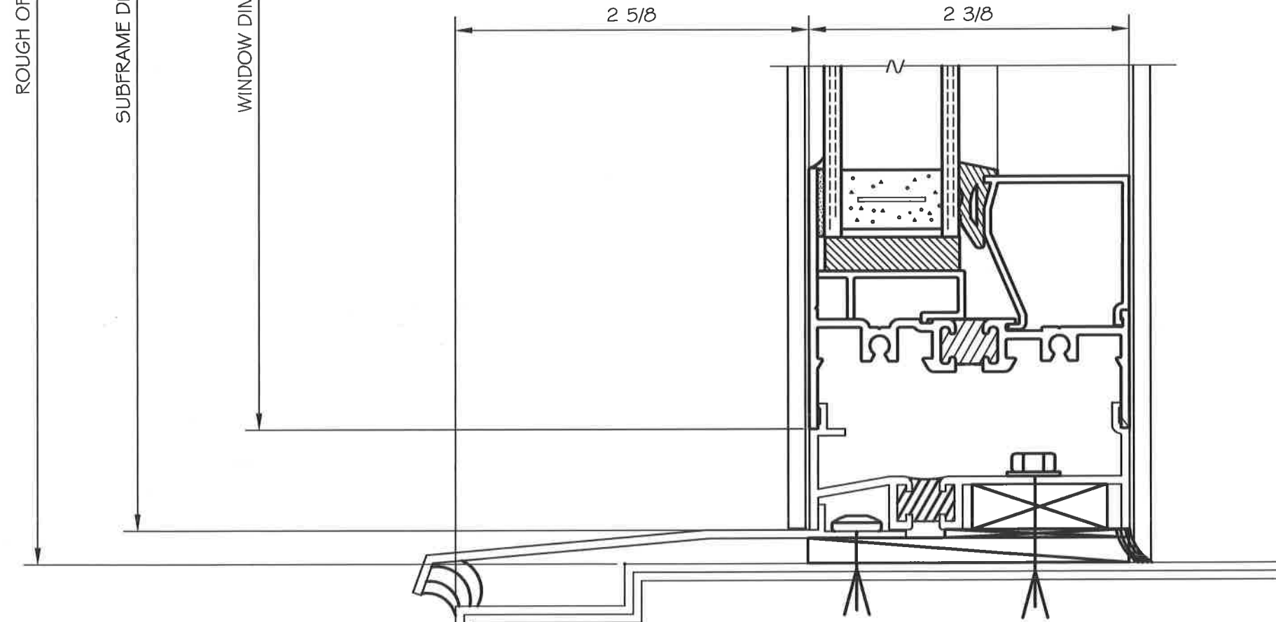
TYPICAL SUBFRAME SILL
