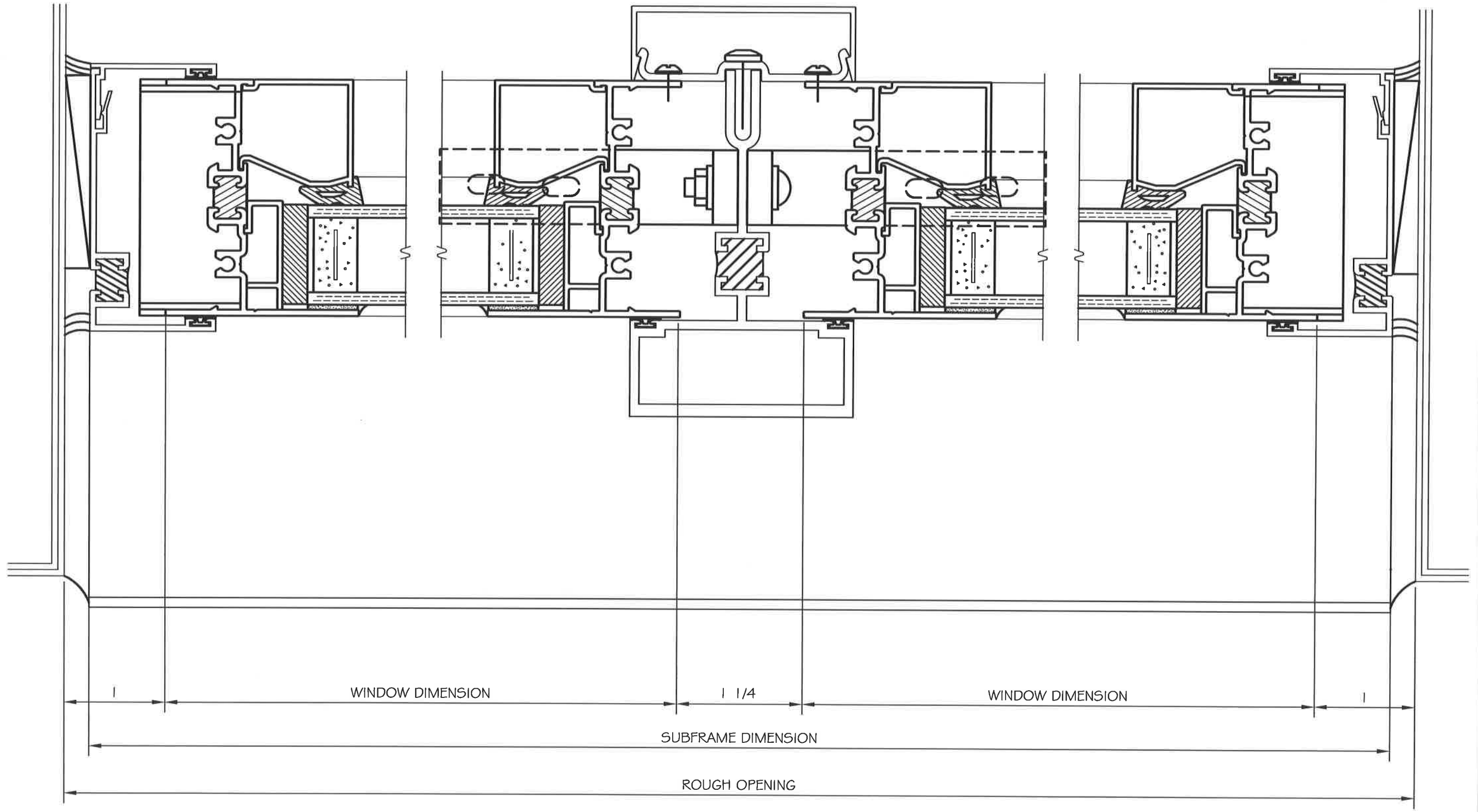
TYPICAL SUBFRAME JAMB
