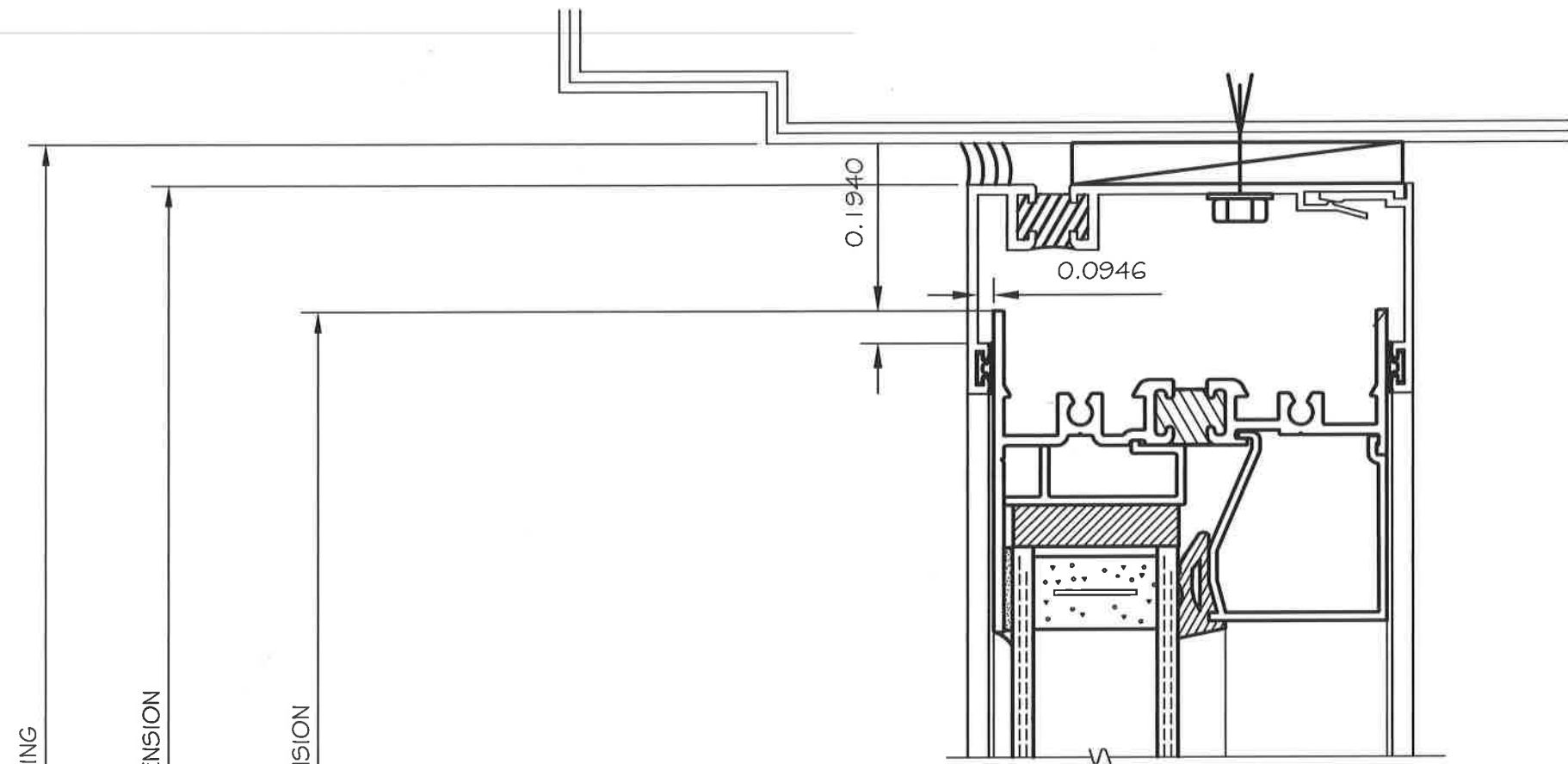
TYPICAL SUBFRAME HEAD
