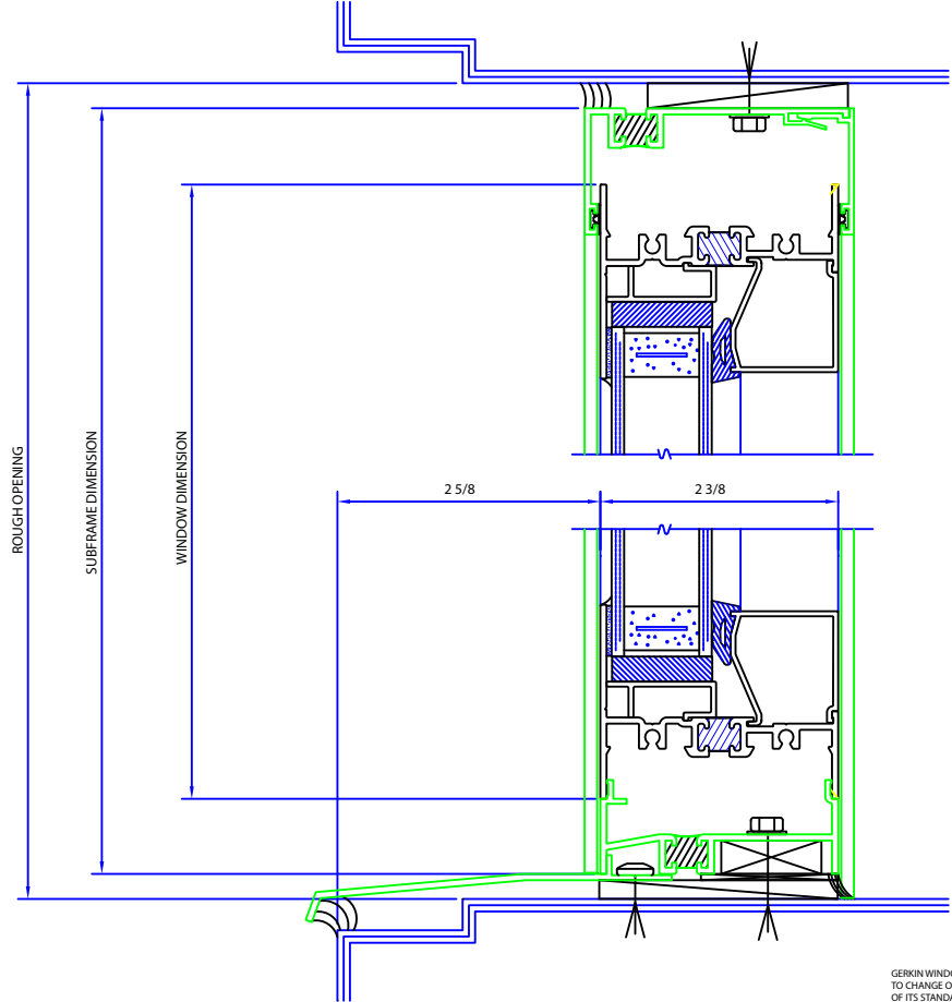
TYPICAL SUBFRAME HEAD
