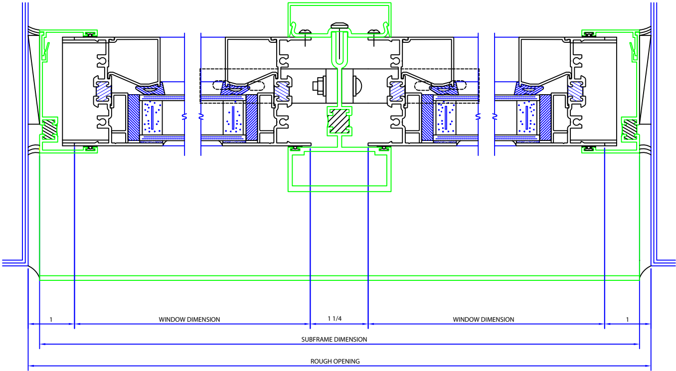
TYPICAL SUBFRAME JAMB
