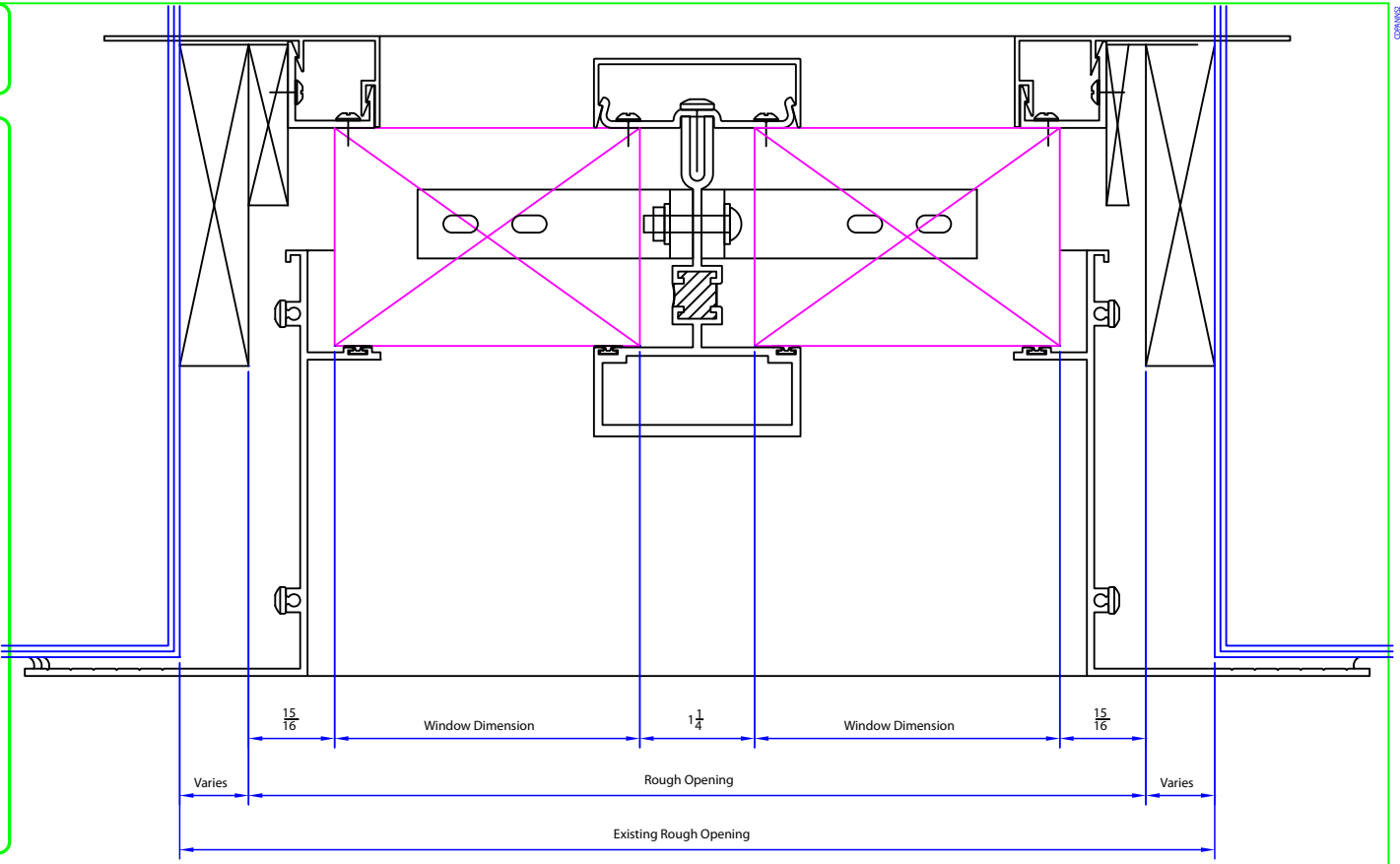
TYPICAL PANNING JAMB
