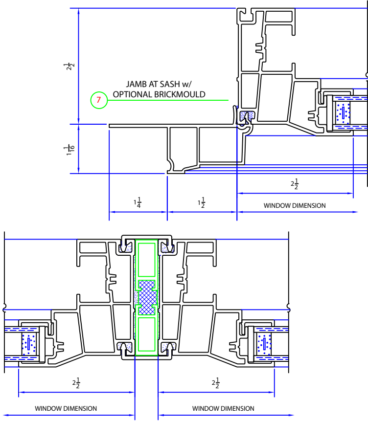
5 TYPICAL MULLION
