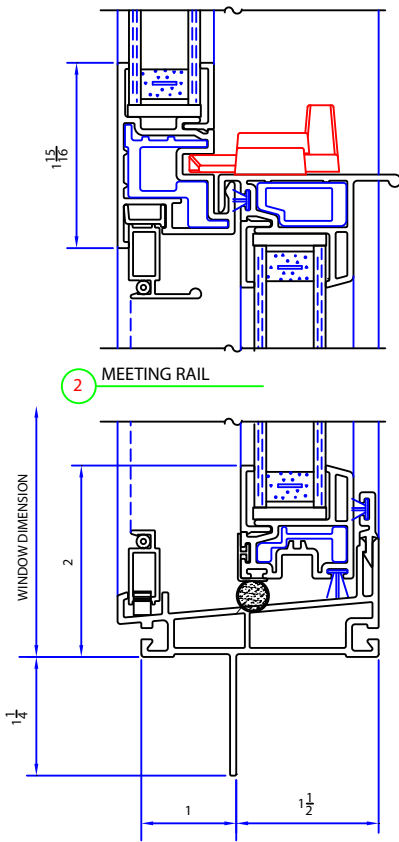
1 TYP. SILL AT SASH
