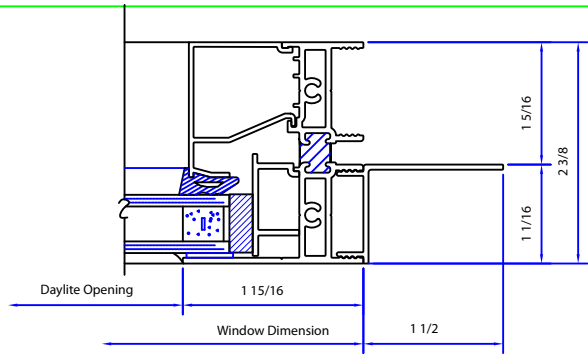
6A JAMB AT FIXED W/ 5/8" GLAZING
