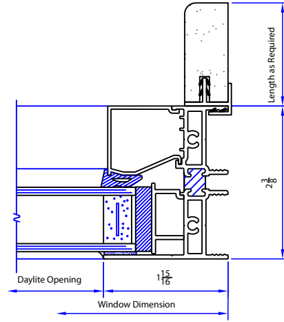
6 JAMB AT FIXED W/ OPTIONAL EXTENSION JAMB
